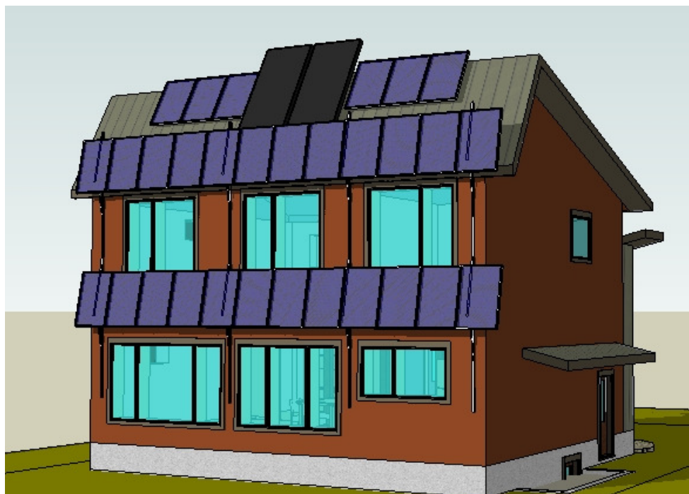
Figure 3. Computer drawing of the south side of the house – with the awning in the winter position
